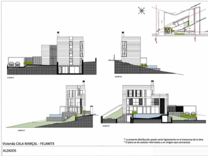
Floor plan
