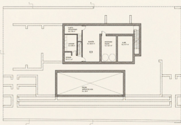
Floor plan (basement)
