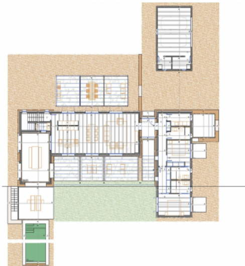
Plans ground floor
