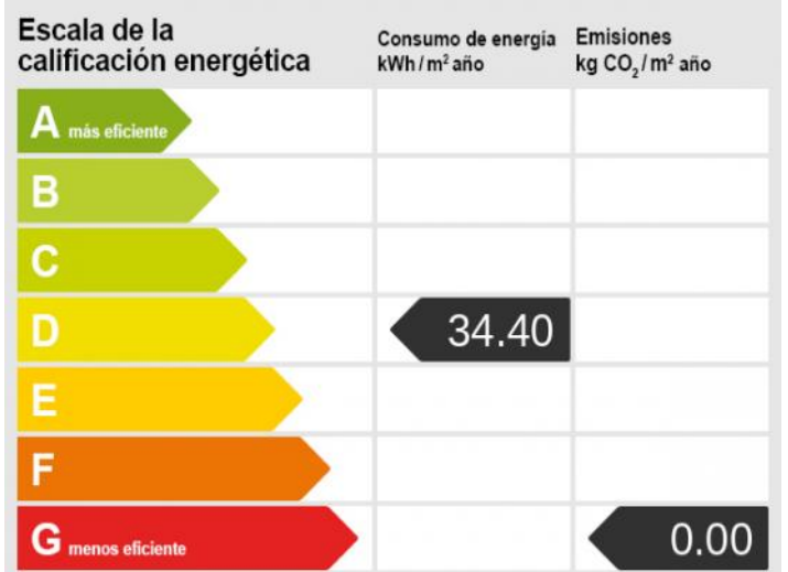
Energy scale
