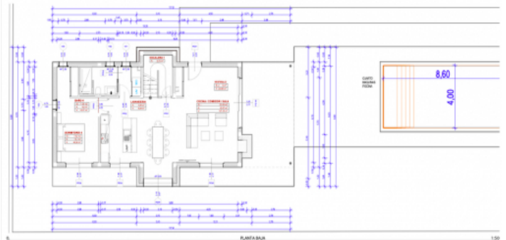
Construction plan
